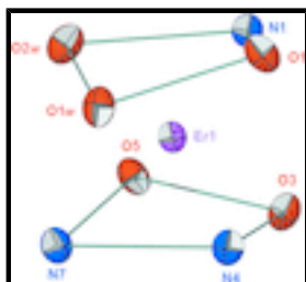
Fig. 2. Square-antiprismatic coordination figure of Er in the title compound.
